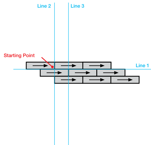
Horizontal Brick
